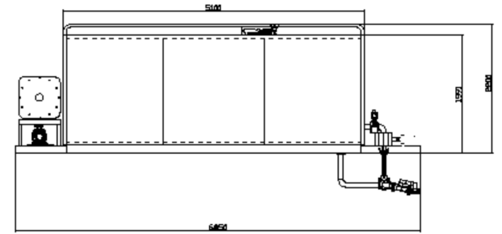
SAMPLE DRAWING FROM RIGHT VIEW ( 14 MS CAPACITY )
