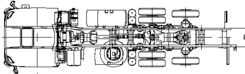
SAMPLE TRUCK DIMENSIONS WITH 80% SWOP BODY
